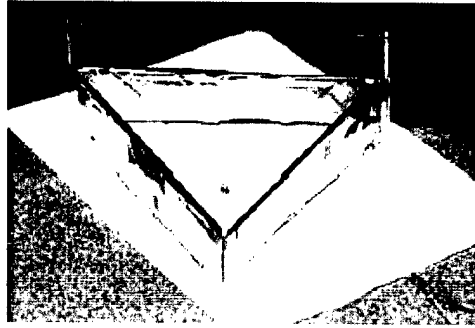
Figure 7. Our first attempt at making an asymmetric capacitor (a “lifter”), according to the specifications given by J. Naudin ( J ) on Internet Web site < http://jnaudin.free.fr/ >.
